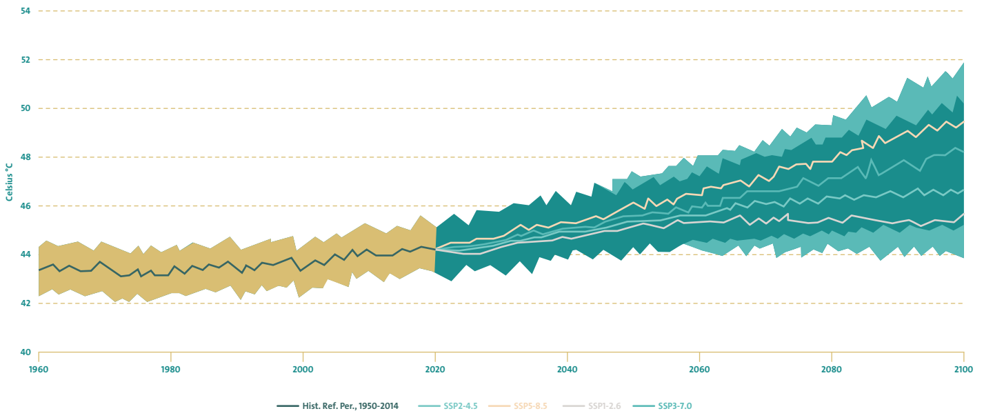
Figure 8: Projected Timeseries Anomaly of Maximum of Daily Max-Temperature, 1950-2100, Multi-Model Ensemble, (Ref. Period: 1995-2014). 19
