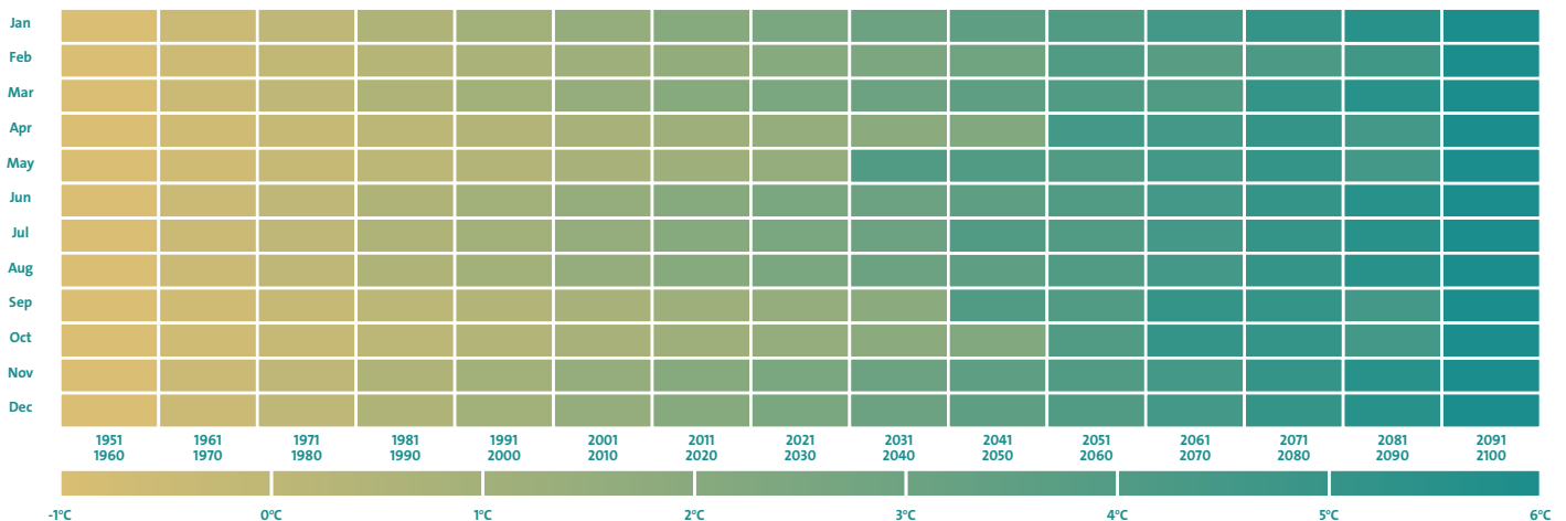
Figure 9: Projected Heat Plot Maximum of Daily Max-Temperature, SSP5-8.5, Multi-Model Ensemble, (Ref. Period: 1995-2014). 19
