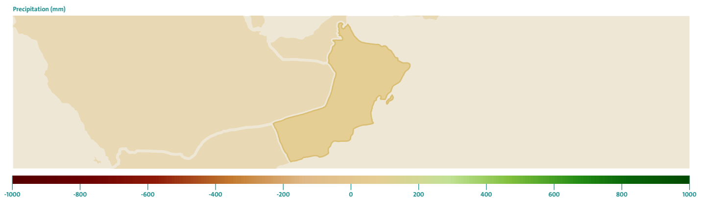
Figure 6: Projected Annual Precipitation Anomaly, 2020-2039, Annual, SSP2-4.5, SSP5-8.5, Multi-Model Ensemble. Ref. Period: 1950-2014. 19
