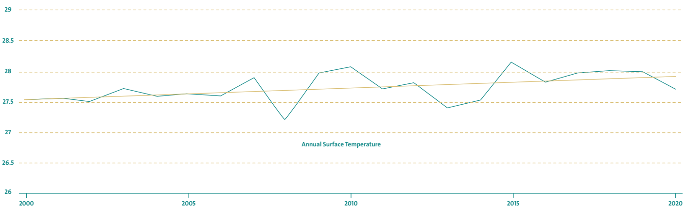
Figure 3: Observed Annual Average Mean Surface Air Temperature Annual Trends with Significant Trend per Decade, Oman 2000-2020 17
