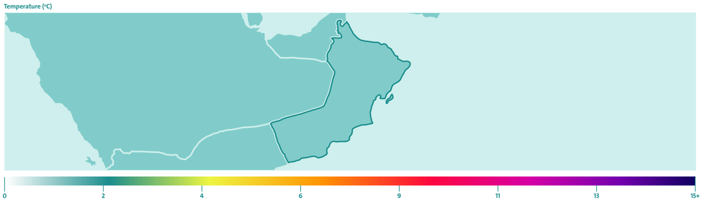
Figure 4: Projected Anomaly of Average Mean Surface Air Temperature, 2080-2099, Annual, SSP5-8.5, Multi-Model Ensemble. Ref. Period: 1995-2014 18
