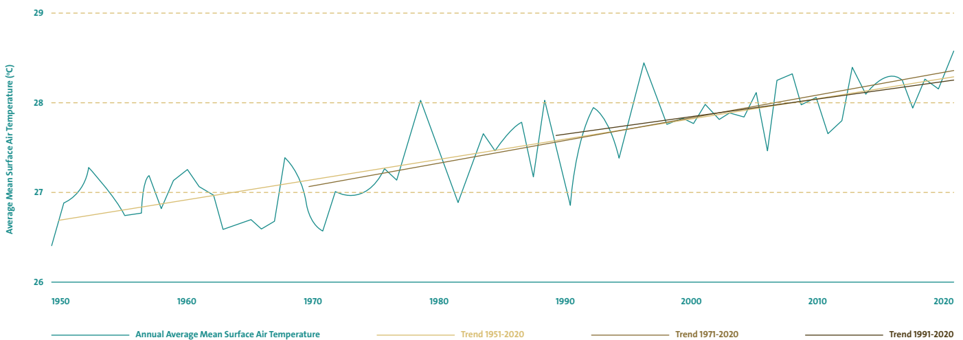
Figure 2: Observed Annual Average Mean Surface Air Temperature with Significant Trend per Decade, Oman 1950-2020 17
