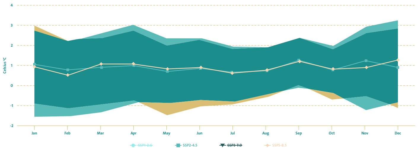
Figure 5: Projected Anomaly of Average Mean Surface Air Temperature, 2080-2099, SSP5-8.5, Multi-Model Ensemble, Ref. Period: 1995-2014 19
