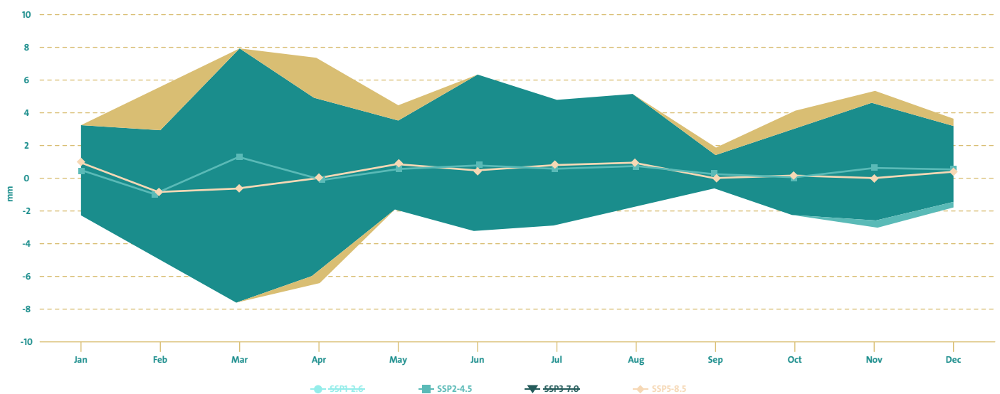
Figure 7: Projected Precipitation Anomaly, 2020-2039, Annual, SSP2-4.5, SSP5-8.5, Multi-Model Ensemble. Ref. Period: 1950-2014. 19
